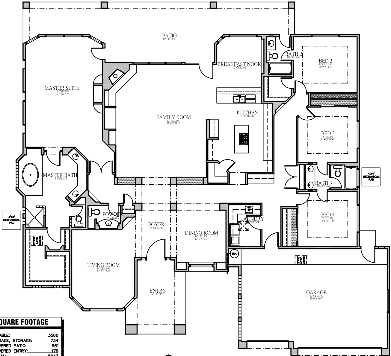
FLOOR PLAN
