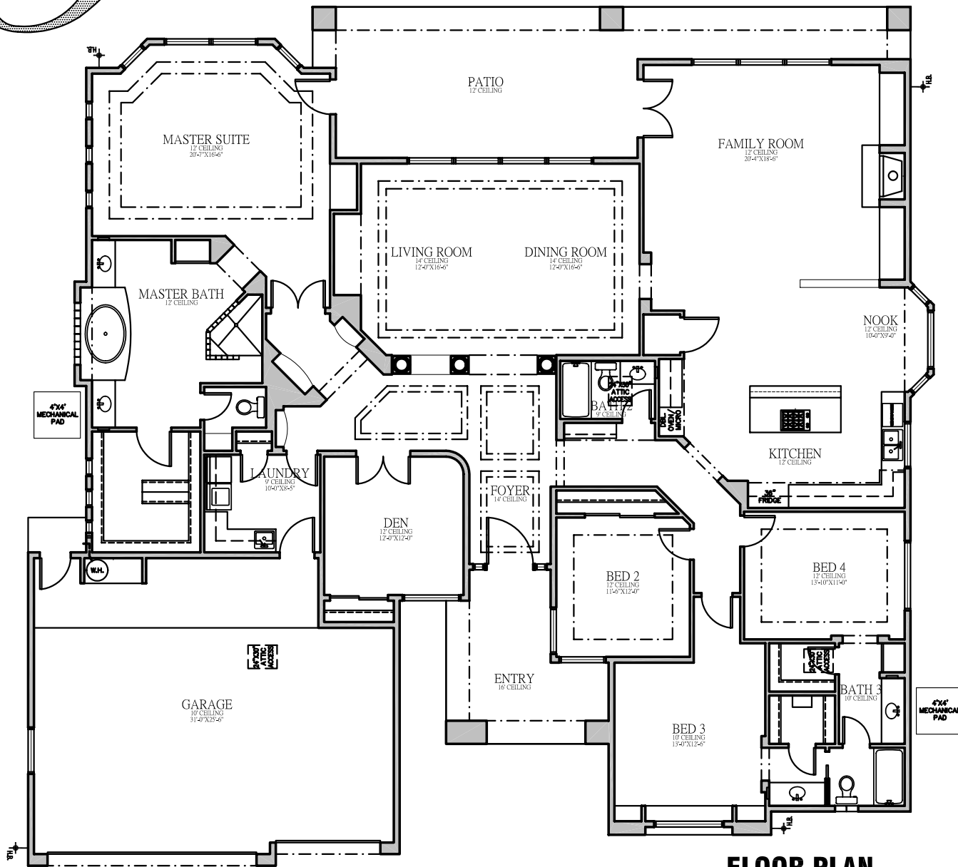
FLOOR PLAN
