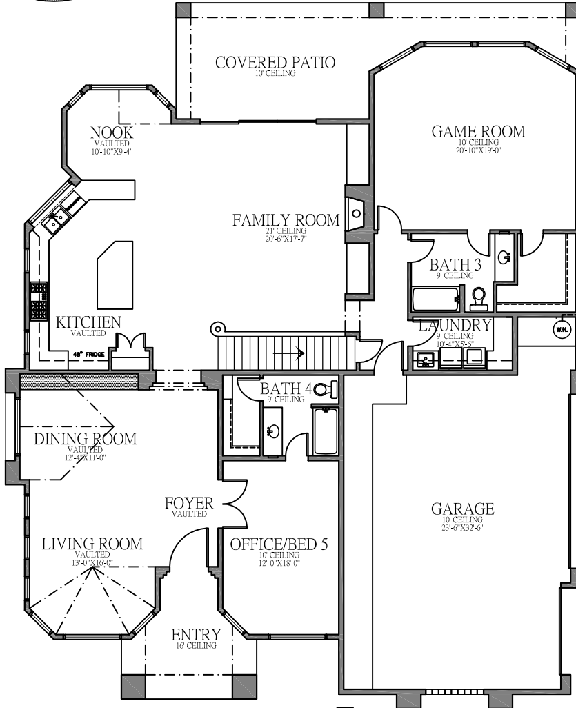
FLOOR PLAN
