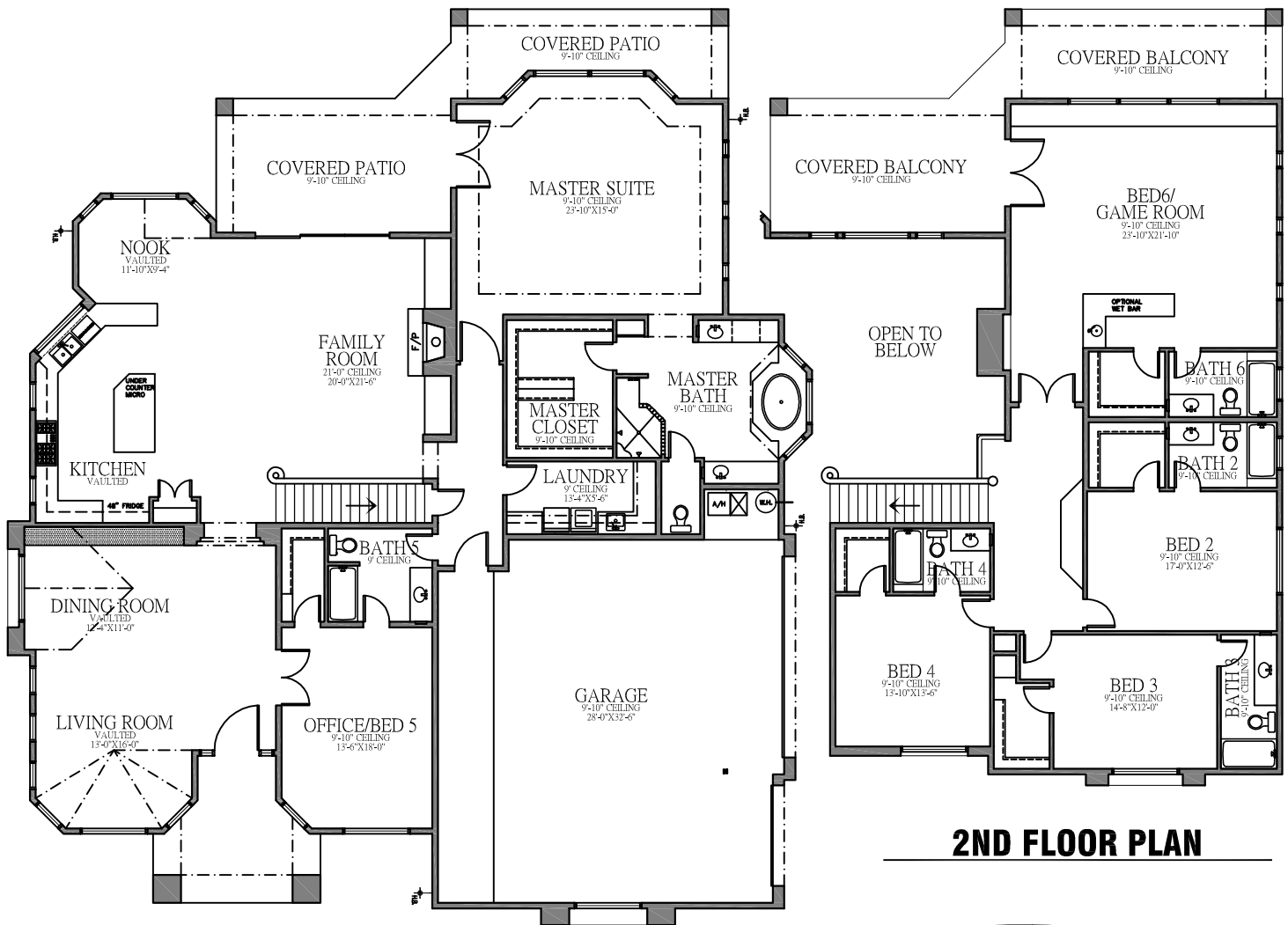
FLOOR PLAN
