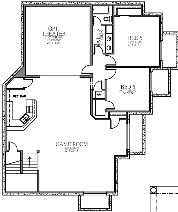
BASEMENT FLOOR PLAN
